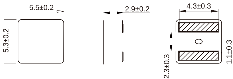
Dimensions: [mm]
