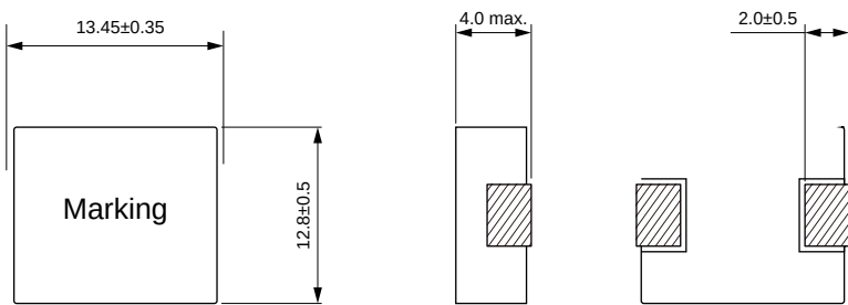
Dimensions: [mm]
