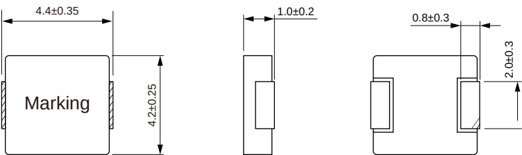
Dimensions: [mm]
