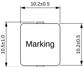
Dimensions: [mm]
